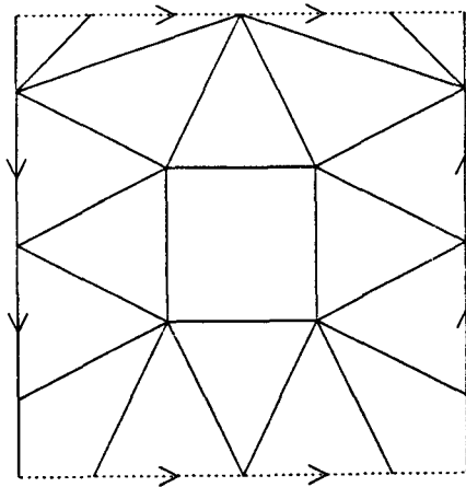
Figure 1. An embedding in the Klein bottle.
